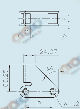
" H " type R/L for 81X
