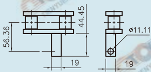
81XH WELDED ATTACHMENT
