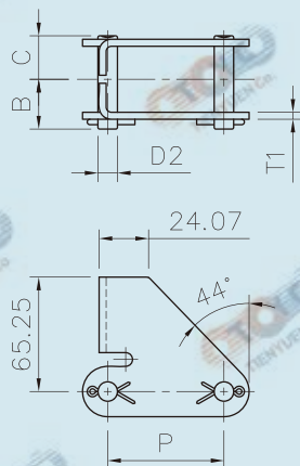
" H " type C/L for 81X
