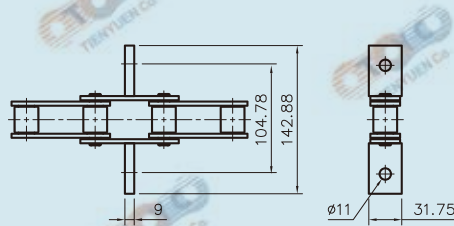
81X WELDED ATTACHMENT
